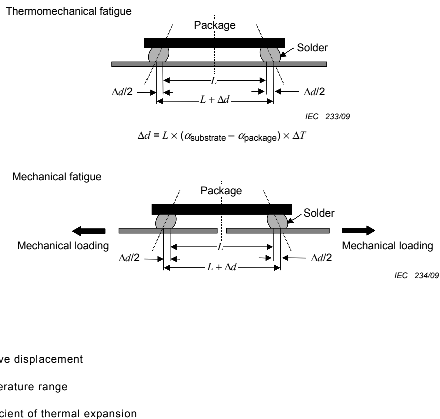
Figure 2 – Schematic illustrations of thermomechanical and mechanical fatigue for solder joints
